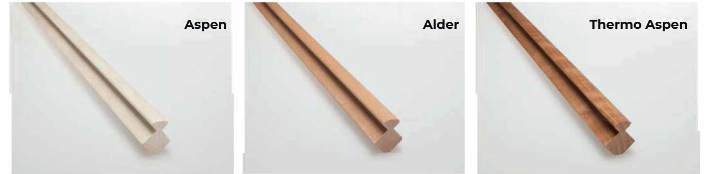
Corner moulding | Thickness: 27 mm | Width: 27 mm | Coverage: 15 mm
